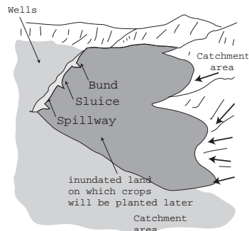
Figure 5.2 Examples of floodwater harvesting techniques.
