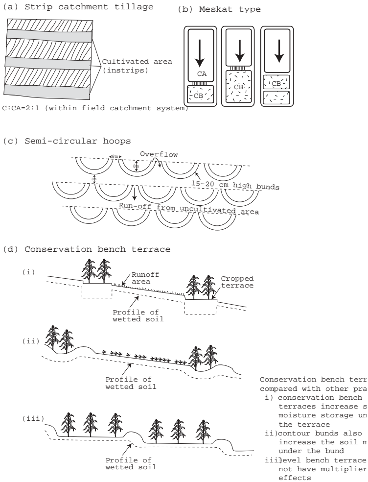
Figure 5.1 Examples of runoff-farming techniques.
