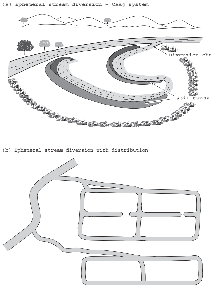
Figure 5.3 Examples of stream flow diversion techniques.
